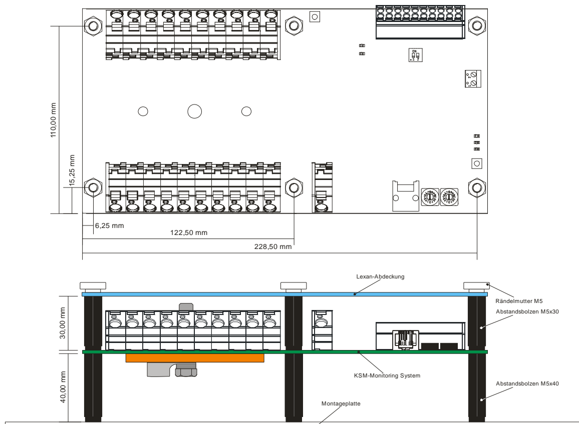
Abb. 2 Montage des KSM-Monitoring Systems
